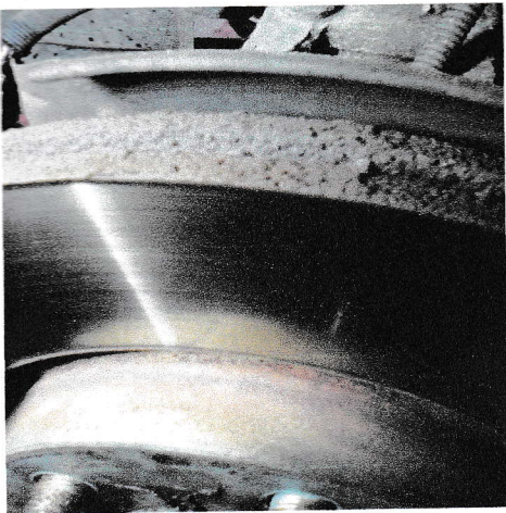
Fig 2 - Supporting Image Visual check of brake discs, shoes and cylinders for wear or damage
