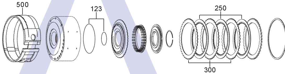
'C3' Clutch Assembly
