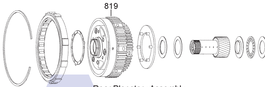
Rear Planetary Assembly
